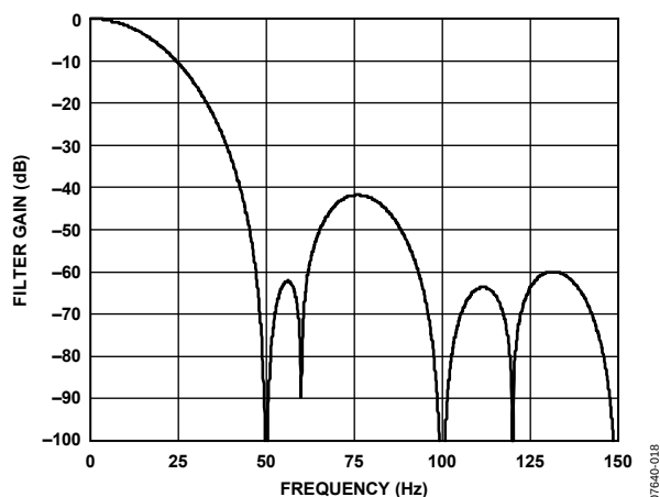
Figure 24. \text{sinc}^3 Filter Response (50 Hz Output Data Rate, REJ60 = 1)
