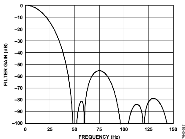
Figure 23. \text{sinc}^4 Filter Response (50 Hz Output Data Rate, REJ60 = 1)
