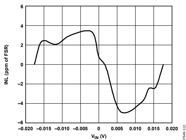
Figure 13. INL (Gain = 128)
