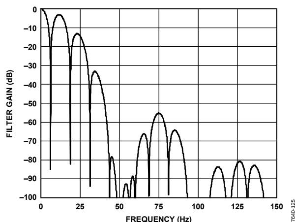
Figure 25. \text{sinc}^4 Filter Response (12.5 Hz Output Data Rate, Chop Enabled, REJ60 = 1)
