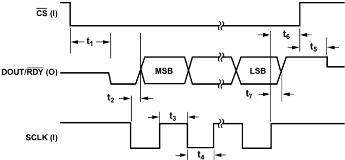
I = INPUT, O = OUTPUT Figure 3. Read Cycle Timing Diagram
