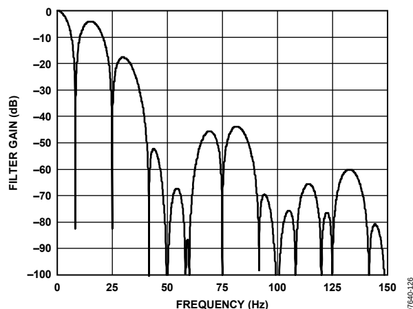
Figure 26. \text{sinc}^3 Filter Response (16.7 Hz Output Data Rate, Chop Enabled, REJ60 = 1)
